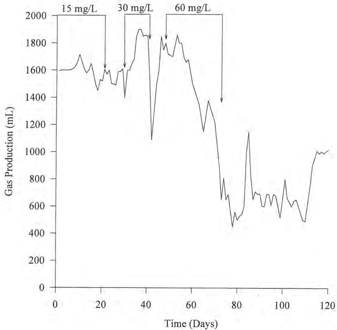
Figure 2. Response of anaerobic filter to an anionic surfactant. (From Yang, et al. 1979)
